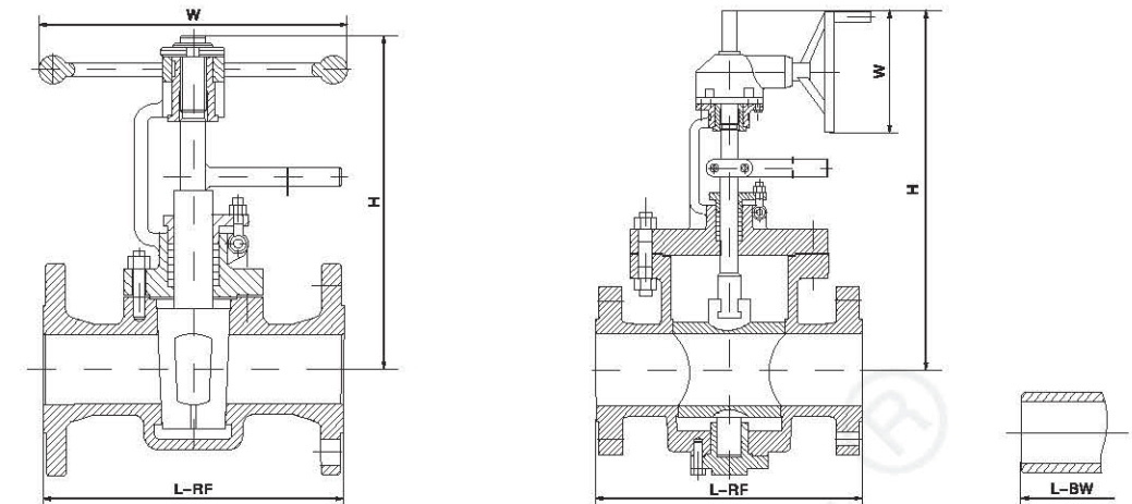
◎主要外形和连接尺寸 Main outline and connecting dimensions
